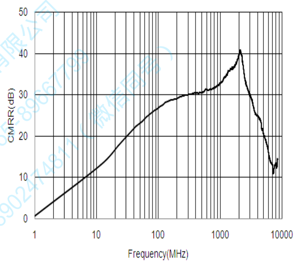
CMRR Characteristics
