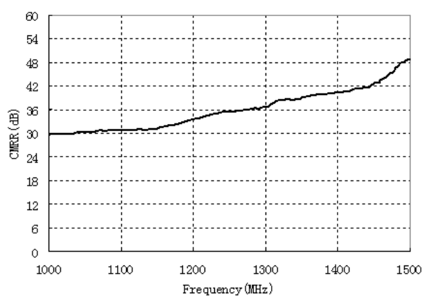
CMRR Characteristics
